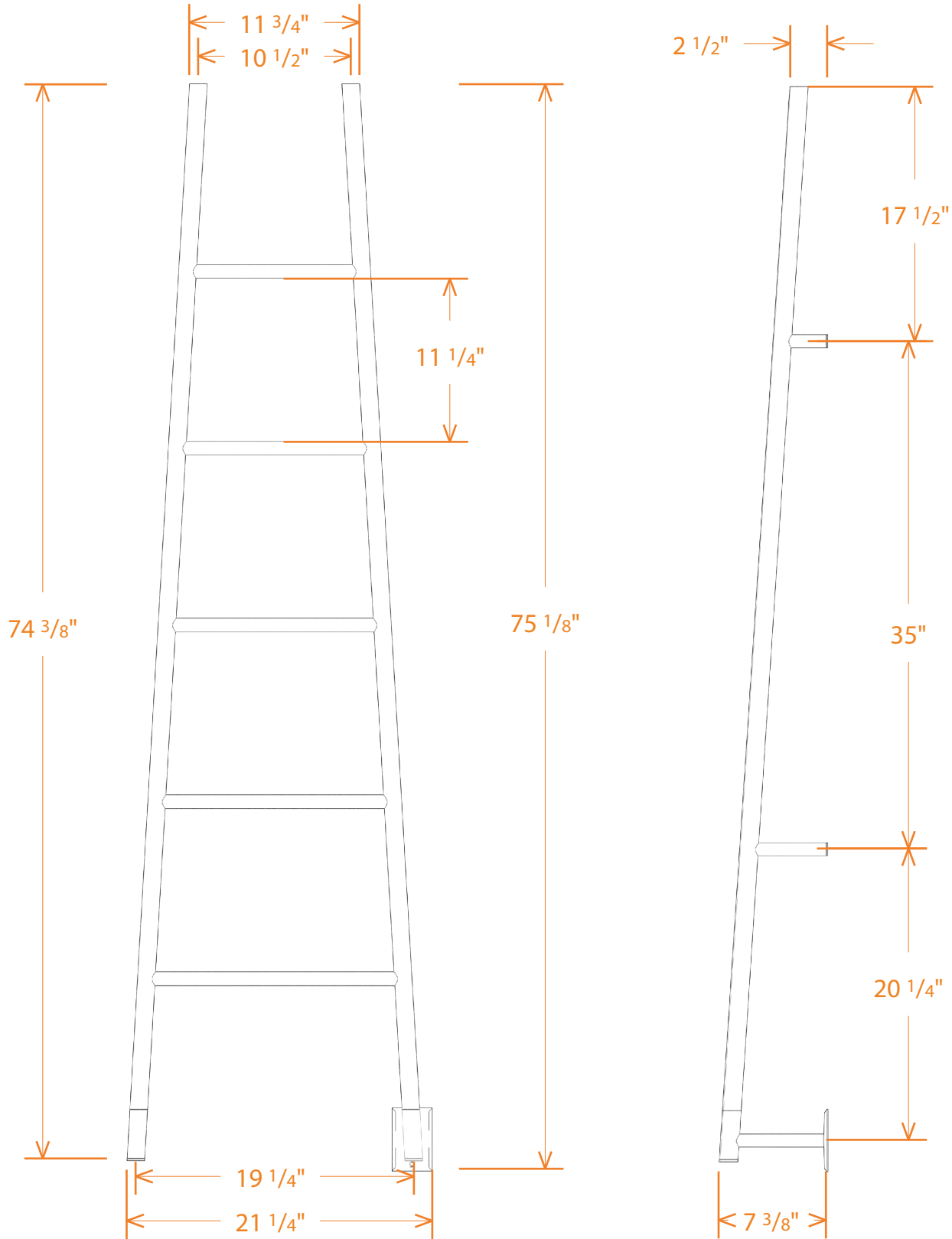
FRONT VIEW OF RACK ON WALL
