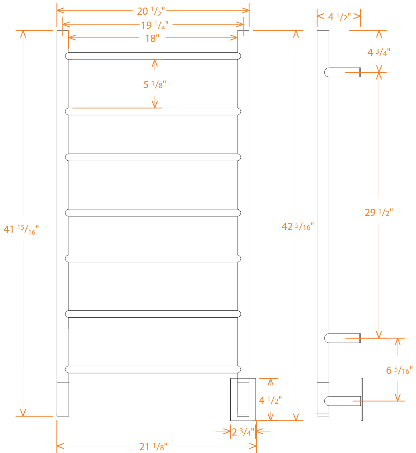
FRONT VIEW OF RACK ON WALL
